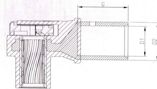
View X-X
