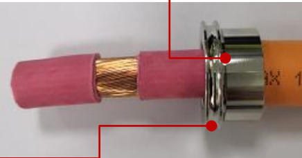
⑧ Outer Copper Ring 外铜环
